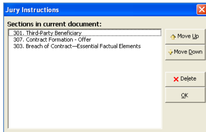
Figure 14 - Arrange/Delete
