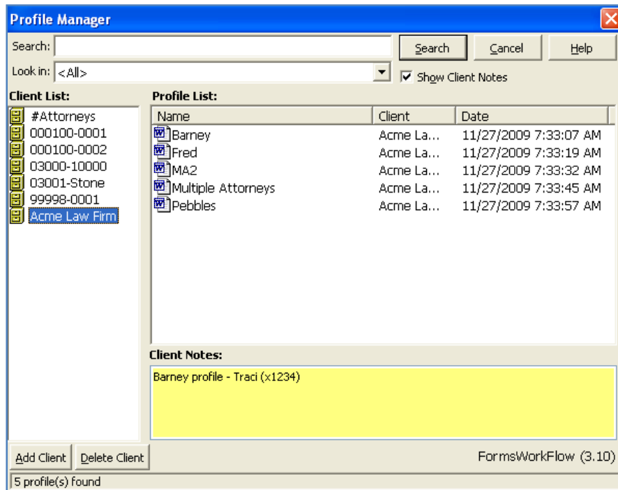
Figure 7 - Profile Manager
