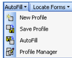
Figure 6 - AutoFill Drop-Down
